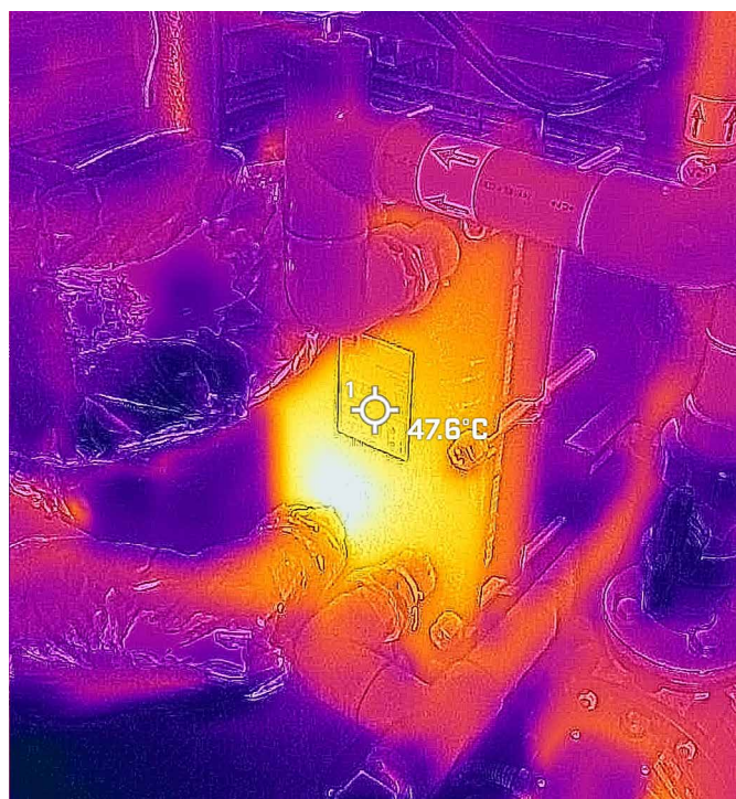
Thermal imaging showing heat loss on a plate heat exchanger
